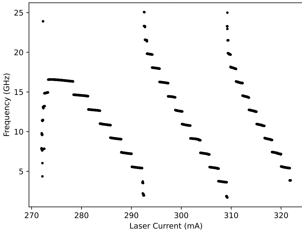
Laser Frequency vs Current
